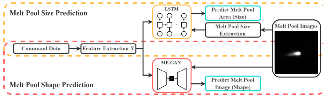
Figure 1. Overall framework for machine learning based prediction of the size and shape of the melt pool.
