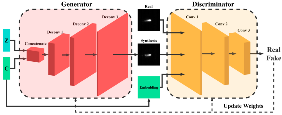
Figure 4. MP-GAN architecture.
