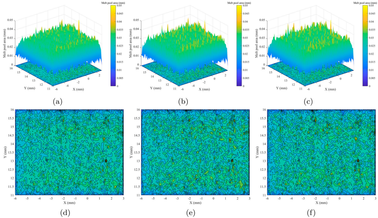
Figure 8. Contour and 3D surface comparison. (a) 3D surface of ground truth. (b) 3D surface of LSTM model. (c) 3D surface of MP-GAN model. (d) Contour plot of ground truth. (e) Contour plot of LSTM model and (f) Contour plot of MP-GAN model.
